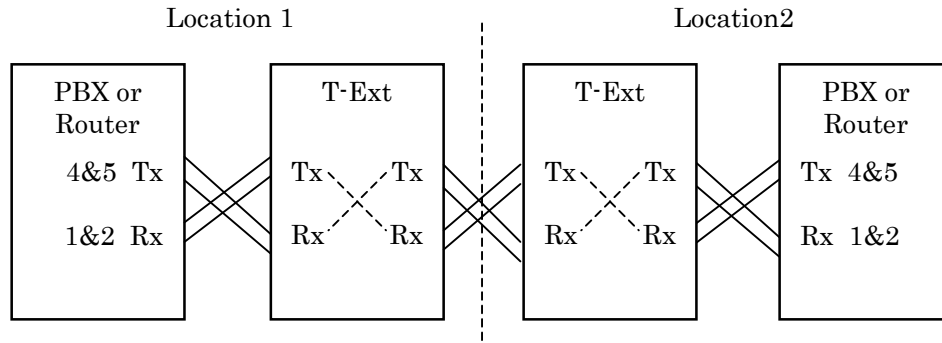
Equipment to Equipment connections.
